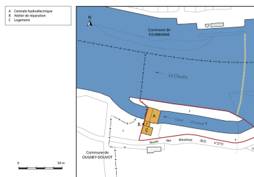
Plan-masse et de situation, section C. Dess. Mathias Papigny IVR43_20142501901NUDA
