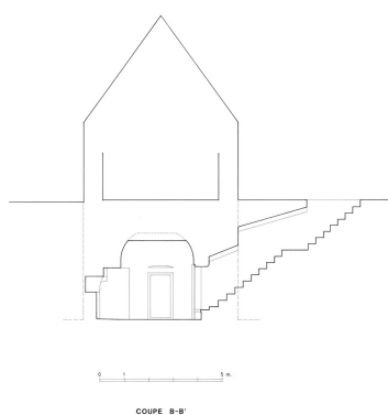
Tour Notre-Dame. Coupe B-B'. Dess. Alain Morelière IVR26_20122100100A2YY
