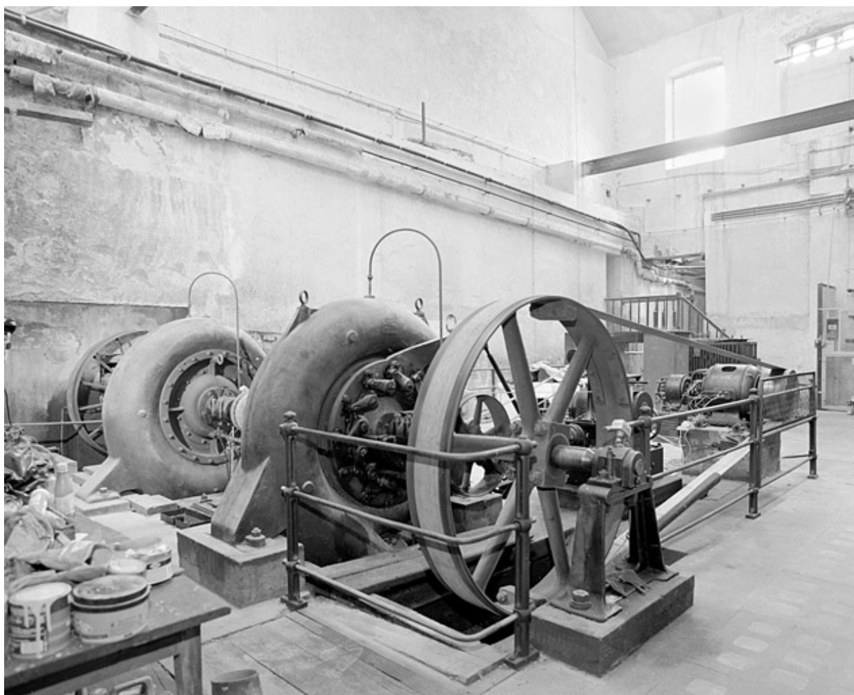
Turbine Francis (1929).
