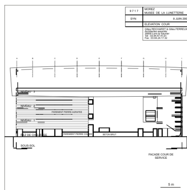
Elévation cour, 2000. Dess. Gilles Reichardt, Dess. Gilles Ferreux, IVR43_20103900241NUDA
