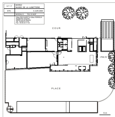
Niveau 0 [plan], 2000. Dess. Gilles Reichardt, Dess. Gilles Ferreux, IVR43_20093900244NUDA
