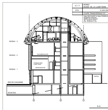
Coupe transversale CC, 2000. Dess. Gilles Reichardt, Dess. Gilles Ferreux, IVR43_20103900149NUDA
