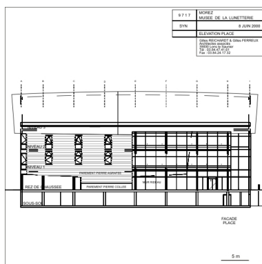
Elévation place, 2000. Dess. Gilles Reichardt, Dess. Gilles Ferreux, IVR43_20103900240NUDA
