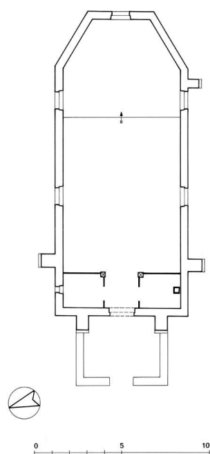
plan Dess. Alain Morelière IVR26_20122100821A2YY
