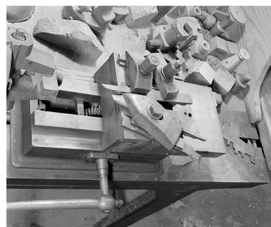
Chariot porte-outil (atelier principal). Phot. Jérôme Mongreville IVR43_20022500634X
