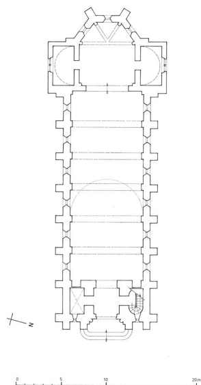
Plan. Dess. Alain Morelière IVR26_20122100511A2YY
