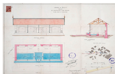
plans du lavoir communal Phot. , Autr. Charles Humbert IVR43_20167001577NUC4A
