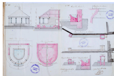
plans de la fontaine "du bas" Phot. , Autr. Jean-Baptiste Ridoux IVR43_20167001580NUC4A
