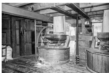
Meules (1979). Phot. J. Dumont IVR43_19792501166Z
