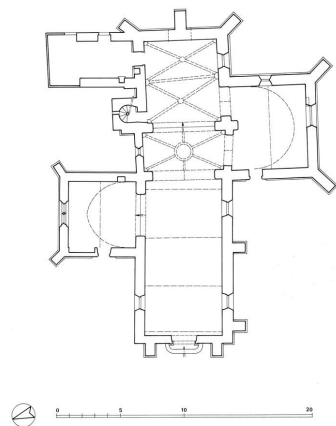
plan Dess. Alain Morelière IVR26_20122100808A2YY
