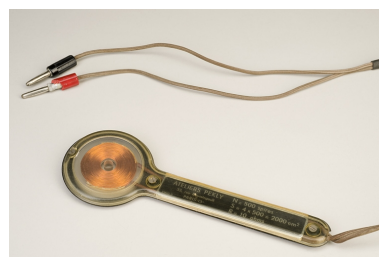
La sonde. Phot. Marc Loukachine IVR43_20122500092NUC4A
