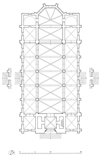
plan Dess. Alain Morelière IVR26_20122100813A2YY
