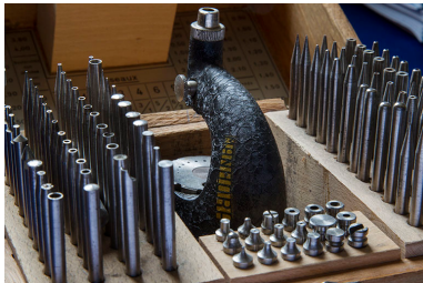
Potence à river Manhora. Phot. Sonia Dourlot IVR43_20142501416NUC2A
