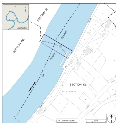
Plan-masse et de situation. Dess. André Céréza IVR43_20062500319NUDA
