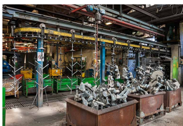
Grenailleuse. Phot. Jérôme Mongreville IVR43_20132500982NUC4A
