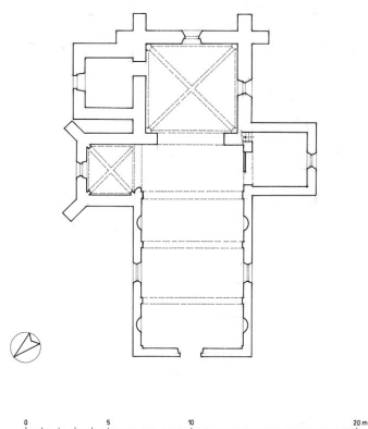
Plan. Dess. Alain Morelière IVR26_20128900009A3YY
