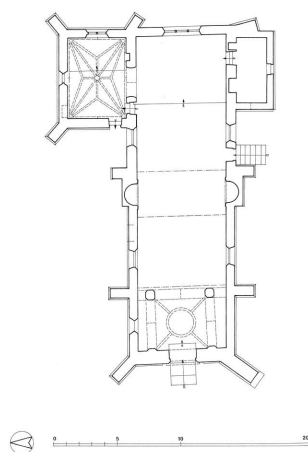
plan Dess. Alain Morelière IVR26_20122100797A2YY
