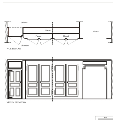
Elévation des boiseries. Dess. André Céréza IVR43_20092501588NUDA
