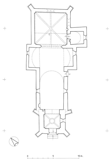
Plan. Dess. Alain Morelière IVR26_20125800110A3YY
