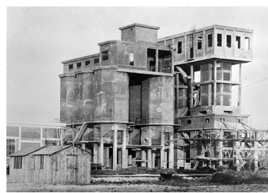
Fours Backmann en construction. Phot. Jérôme Mongreville, Phot. Charnotet IVR43_19903900043X
