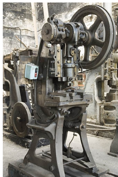
Atelier est. Presse "col de cygne". Phot. Jérôme Mongreville IVR43_20087000834NUC2A
