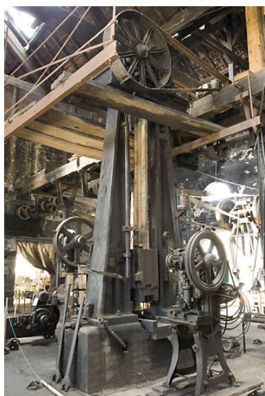
Atelier est. Marteau-pilon Olier et Cie (Clermont-Ferrand). Phot. Jérôme Mongreville IVR43_20087000835NUC2A
