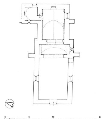
plan Dess. Alain Morelière IVR26_20122100004A3YY
